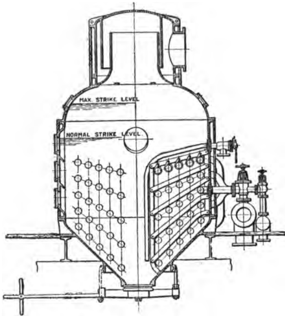
FIG. 27.—COIL-PAN 1
